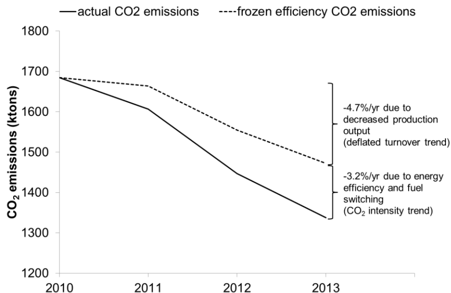
Figure 4: Actual and frozen efficiency CO 2 emissions in the period 2010-2013 (n = 50).
